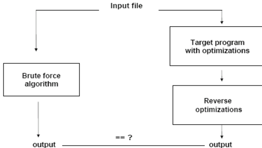
Figure 8-1: Visualization of the oracle approach to verification.
