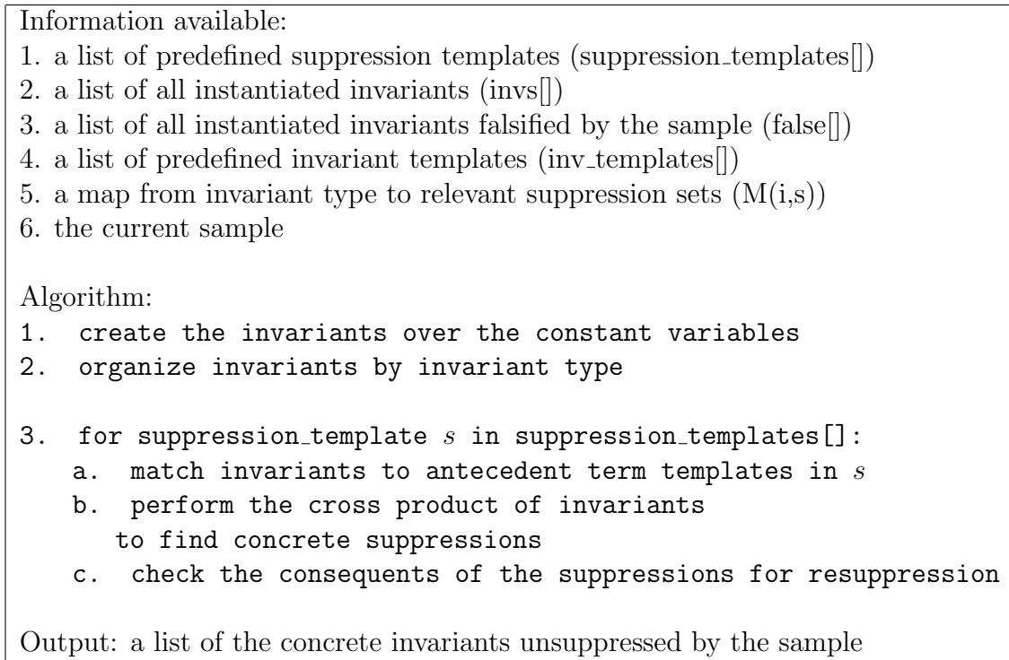
Figure 4-1: Pseudocode for the antecedents algorithm.
